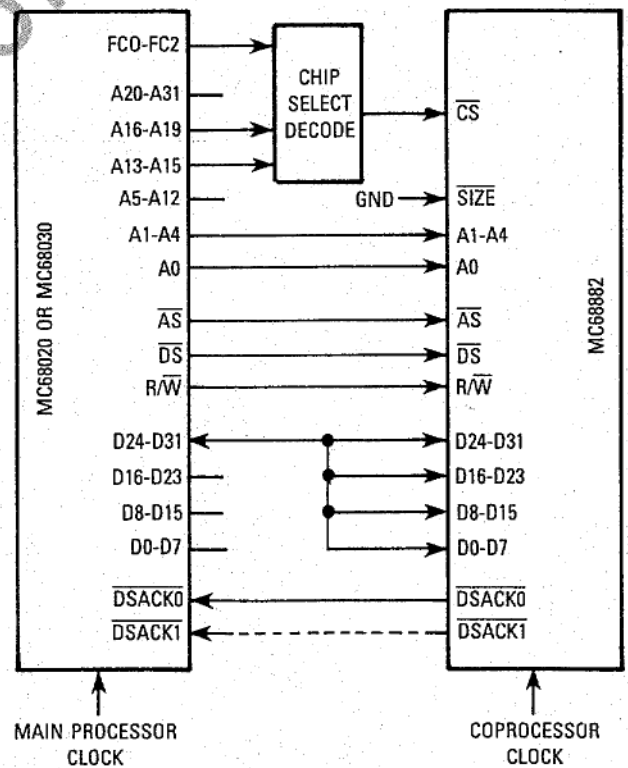
Figure 13. 8-Bit Data Bus Coprocessor Connection
