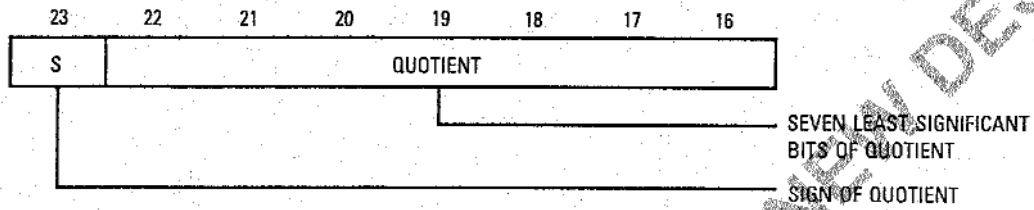
Figure 5. Quotient Byte
