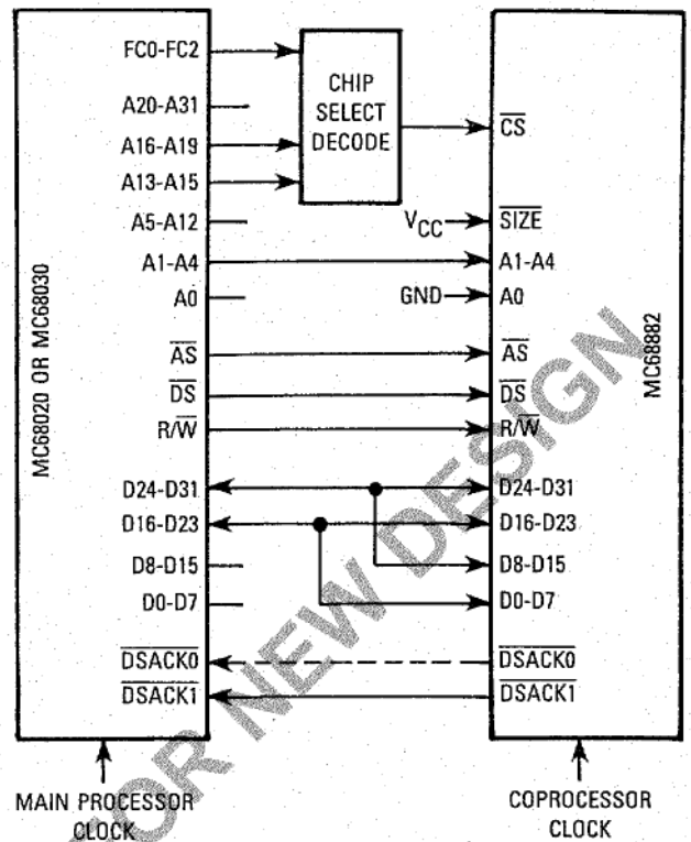
Figure 12. 16-Bit Data Bus Coprocessor Connection
