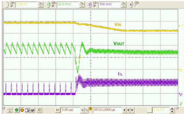
Figure 22. Combined Line / Load Transient, 3.9-3.3 V_{IN} , 10 \mu\text{s} Edge, 36-400 mA Load, 100 ns Edge
