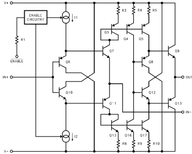
Simplified Schematic (per Amplifier)
