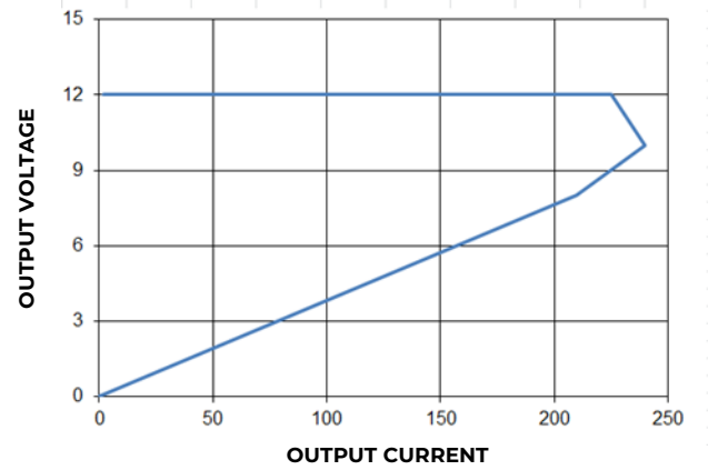
Figure 2. 12V output : Current limit profile ( V_{in} : -48V_{dc} )
